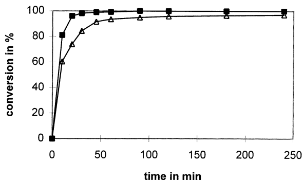
Fig. 6. Suzuki reaction of 15 mmol phenylboronic acid with 13.5 mmol p -iodoanisole in 45 ml water; catalyst: 0.01 mmol \text{PdCl}_2[\text{Ph}_2\text{P}(\text{CH}_2)_4\text{SO}_3\text{K}]_2 . CTAB as micelle forming reagent and 45 mmol \text{Na}_2\text{CO}_3 as base. Ratio iodoanisole: CTAB (I:C) = 1 or 4, at 78°C.
